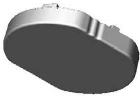
Paint Mask
